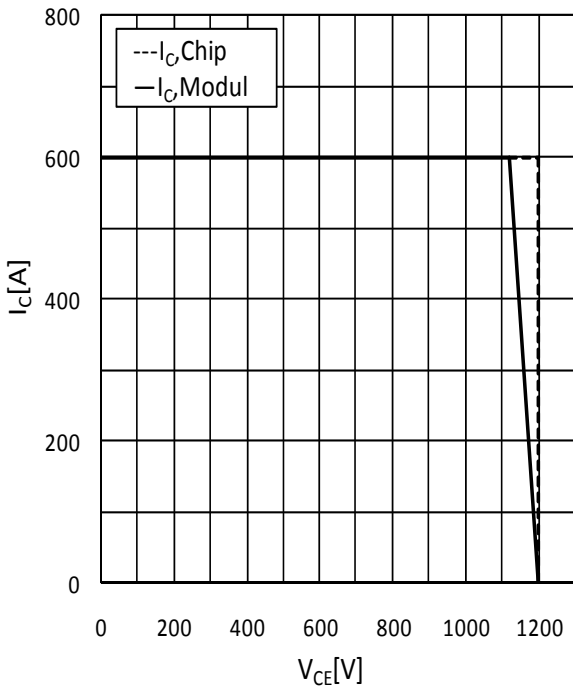
Fig.15 Reverse Bias Safe Operating Area (RBSOA)
